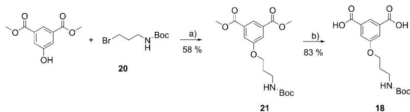
Scheme 3. Synthesis of alkylated isophthalic acid 18 . a) \text{K}_2\text{CO}_3 , acetone, reflux overnight; b) \text{LiOH} , \text{THF}/\text{H}_2\text{O} 1:1, 48 h.
