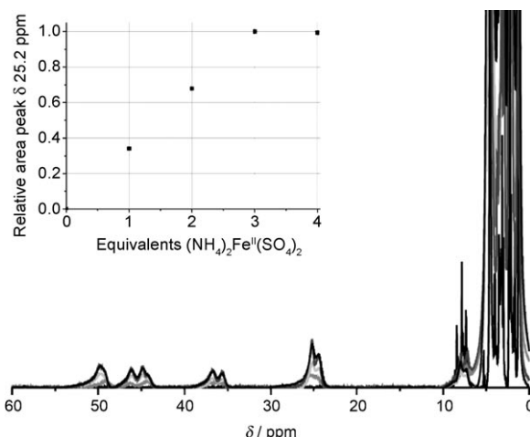
Figure 2. ^1\text{H} NMR titration of 7 in \text{D}_2\text{O} with (\text{NH}_4)_2\text{Fe}^{\text{II}}(\text{SO}_4)_2 (—) 0 equiv \text{Fe}^{\text{II}} , (—) 1 equiv \text{Fe}^{\text{II}} , (—) 2 equiv \text{Fe}^{\text{II}} , (—) 3 equiv \text{Fe}^{\text{II}} , and (—) 4 equiv \text{Fe}^{\text{II}} . Inset: Plot of the relative area of the absorption at \delta = 25.2 ppm compared to the acetone peak against the number of equivalents of (\text{NH}_4)_2\text{Fe}(\text{SO}_4)_2 .
