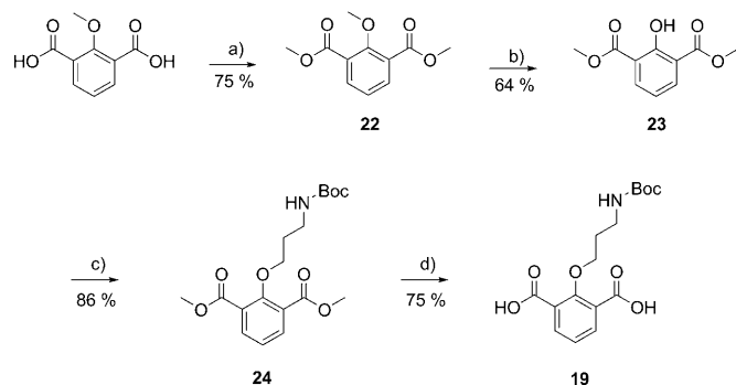
Scheme 4. Synthesis of alkylated isophthalic acid 19 . a) conc. \text{H}_2\text{SO}_4 , \text{MeOH} , overnight; b) \text{BBr}_3 , \text{CH}_2\text{Cl}_2 , -78^\circ\text{C} , 45 min; c) 20 , \text{K}_2\text{CO}_3 , \text{DMF} , reflux overnight; d) \text{LiOH} , \text{THF}/\text{H}_2\text{O} 1:1, 24 h.
